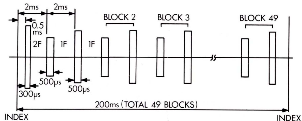
Fig.1 Waveform of T19 (Servo pattern) (T39, 119)
