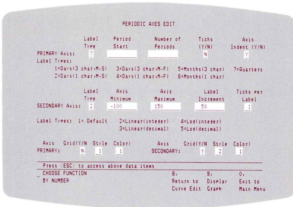
Figure 4-12. PERIODIC AXES EDIT Menu
