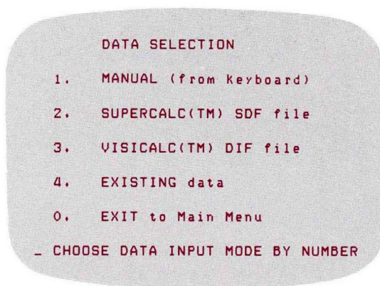
Figure 6-4. DATA SELECTION Menu
